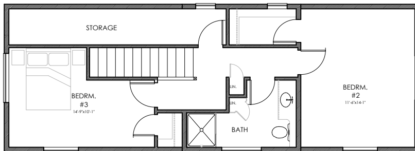
TOP LEVEL PLAN
