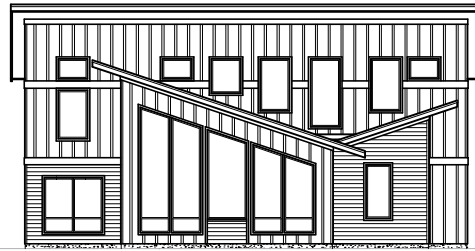
SIDE ELEVATION
