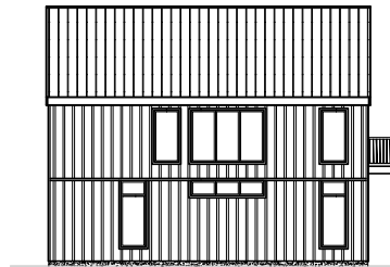
ELEVATIONS
